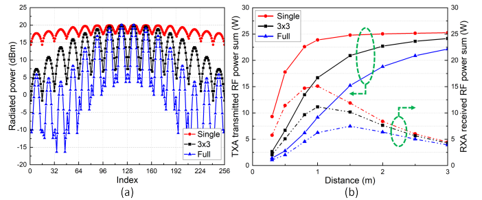
Fig. 6. (a) Radiated power (dBm) of TXA plotted by 1D index with 20 dBm normalization, (b) TXA/RXA RF power sum (W) plotting by distance (m).
