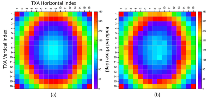
Fig. 17. Heatmap of TXA radiation phase distribution by CVX pattern implementation, with units in degrees. (a) Ideal pattern. (b) LUT-read pattern.
