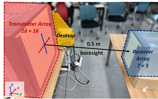
Fig. 15. Full-system configuration.
