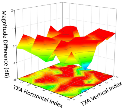
Fig. 14. Magnitude difference of the LUT-based simulation received power and measured power, units in dB.
